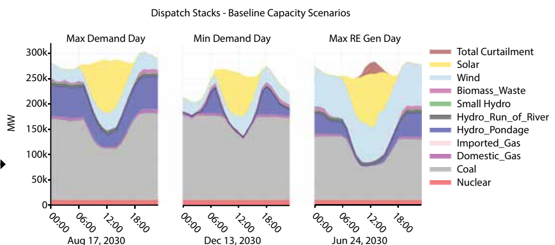
Figure 5: All-India Dispatch Stacks in the Baseline Capacity, Baseline Flexibility Scenario
