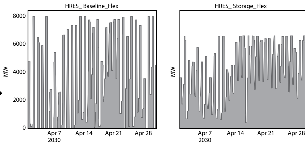
Figure 11: Hourly Dispatch of the 20 Most-Aggressively- Cycled Coal Units
